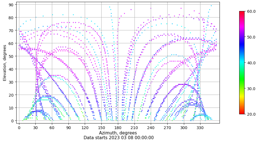
Azimuth-elevation plot for station ALBA. Signal to Noise S1C Data file ALBA00ESP_R_2023067.xtr
