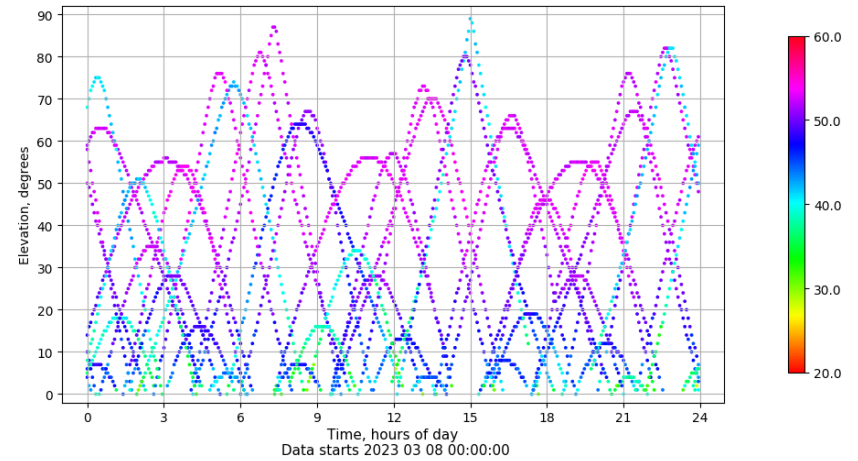
Time-elevation plot for station ALBA. Signal to Noise S1C Data file ALBA00ESP_R_2023067.xtr
