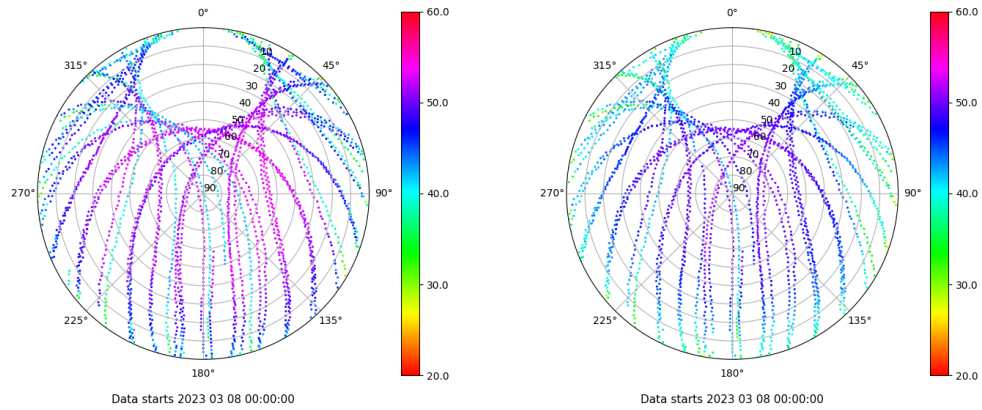
Skyplot for station ALBA. Signal to Noise S1C Data file ALBA00ESP_R_2023067.xtr Skyplot for station ALBA. Signal to Noise S2C Data file ALBA00ESP_R_2023067.xtr
