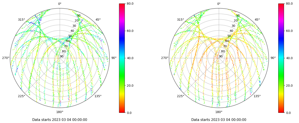
Skyplot for station ALBA. Parameter M1C Data file ALBA00ESP_R_2023063.xtr Skyplot for station ALBA. Parameter M2C Data file ALBA00ESP_R_2023063.xtr
