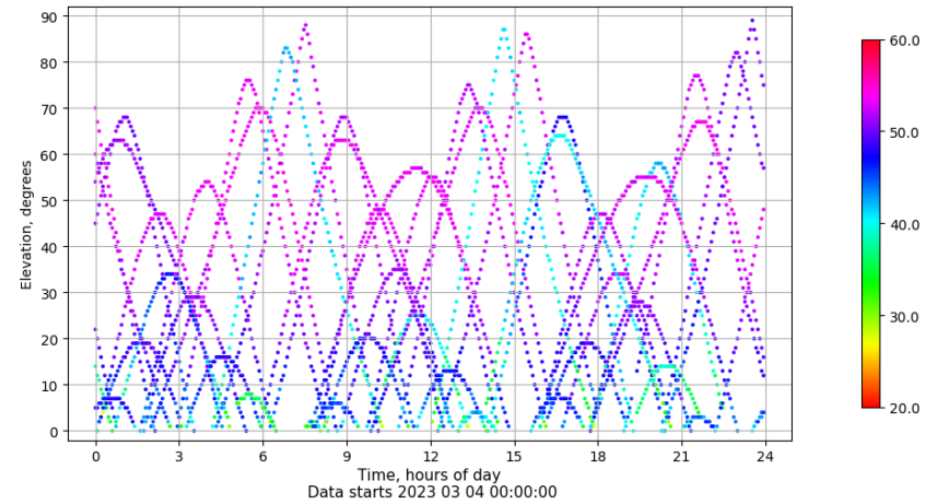
Time-elevation plot for station ALBA. Signal to Noise S1C Data file ALBA00ESP_R_2023063.xtr
