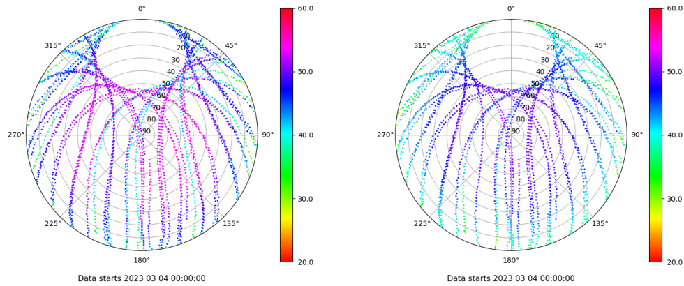
Skyplot for station ALBA. Signal to Noise S1C Data file ALBA00ESP_R_2023063.xtr Skyplot for station ALBA. Signal to Noise S2C Data file ALBA00ESP_R_2023063.xtr
