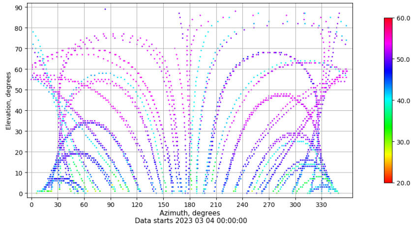
Azimuth-elevation plot for station ALBA. Signal to Noise S1C Data file ALBA00ESP_R_2023063.xtr
