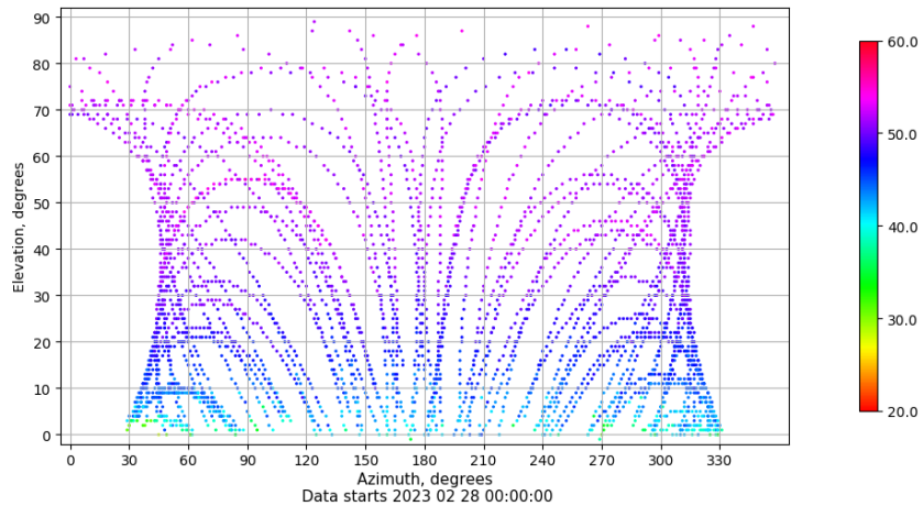
Azimuth-elevation plot for station ALBA. Signal to Noise S1C Data file ALBA00ESP_R_2023059.xtr
