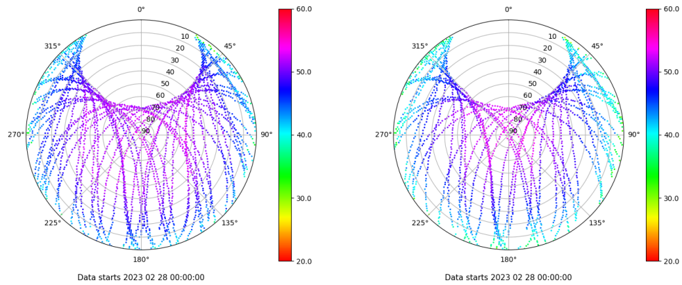
Skyplot for station ALBA. Signal to Noise S1C Data file ALBA00ESP_R_2023059.xtr Skyplot for station ALBA. Signal to Noise S2S Data file ALBA00ESP_R_2023059.xtr
