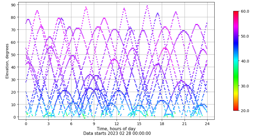
Time-elevation plot for station ALBA. Signal to Noise S1C Data file ALBA00ESP_R_2023059.xtr
