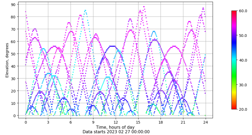
Time-elevation plot for station ALBA. Signal to Noise S1C Data file ALBA00ESP_R_2023058.xtr
