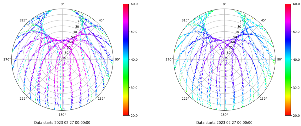
Skyplot for station ALBA. Signal to Noise S1C Data file ALBA00ESP_R_2023058.xtr Skyplot for station ALBA. Signal to Noise S2C Data file ALBA00ESP_R_2023058.xtr
