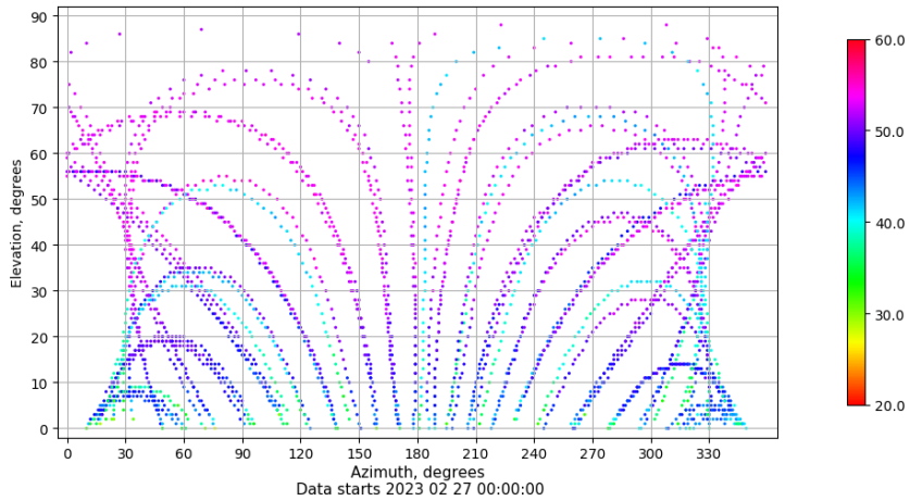
Azimuth-elevation plot for station ALBA. Signal to Noise S1C Data file ALBA00ESP_R_2023058.xtr
