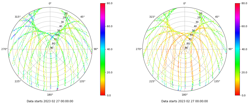
Skyplot for station ALBA. Parameter M1C Data file ALBA00ESP_R_2023058.xtr Skyplot for station ALBA. Parameter M2C Data file ALBA00ESP_R_2023058.xtr
