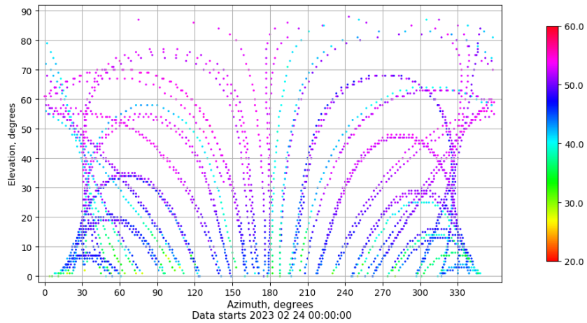
Azimuth-elevation plot for station ALBA. Signal to Noise S1C Data file ALBA00ESP_R_2023055.xtr
