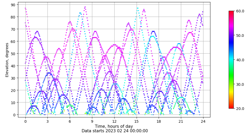
Time-elevation plot for station ALBA. Signal to Noise S1C Data file ALBA00ESP_R_2023055.xtr
