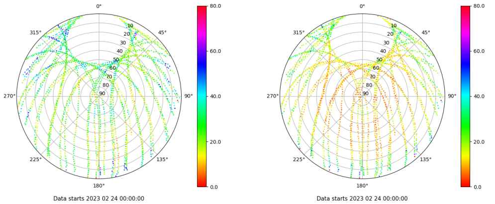
Skyplot for station ALBA. Parameter M1C Data file ALBA00ESP_R_2023055.xtr Skyplot for station ALBA. Parameter M2C Data file ALBA00ESP_R_2023055.xtr
