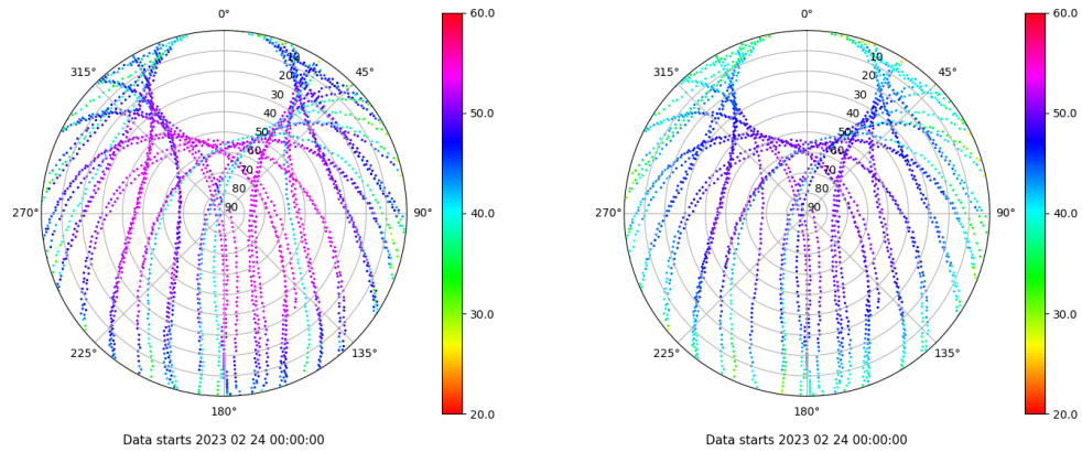
Skyplot for station ALBA. Signal to Noise S1C Data file ALBA00ESP_R_2023055.xtr Skyplot for station ALBA. Signal to Noise S2C Data file ALBA00ESP_R_2023055.xtr
