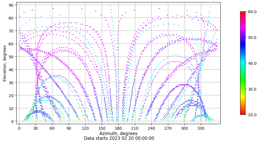
Azimuth-elevation plot for station ALBA. Signal to Noise S1C Data file ALBA00ESP_R_2023051.xtr
