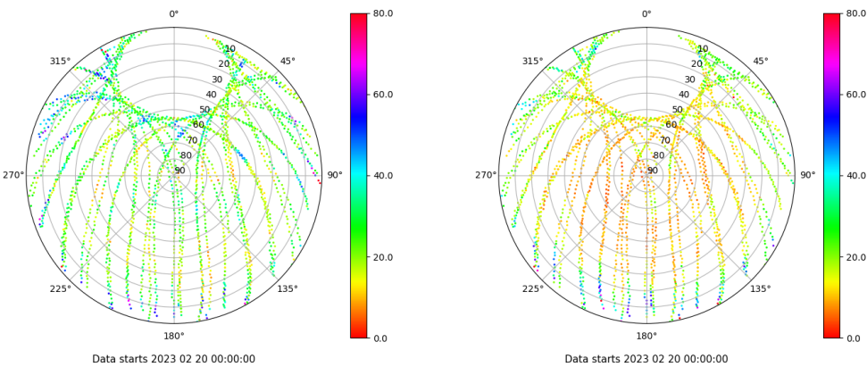
Skyplot for station ALBA. Parameter M1C Data file ALBA00ESP_R_2023051.xtr Skyplot for station ALBA. Parameter M2C Data file ALBA00ESP_R_2023051.xtr
