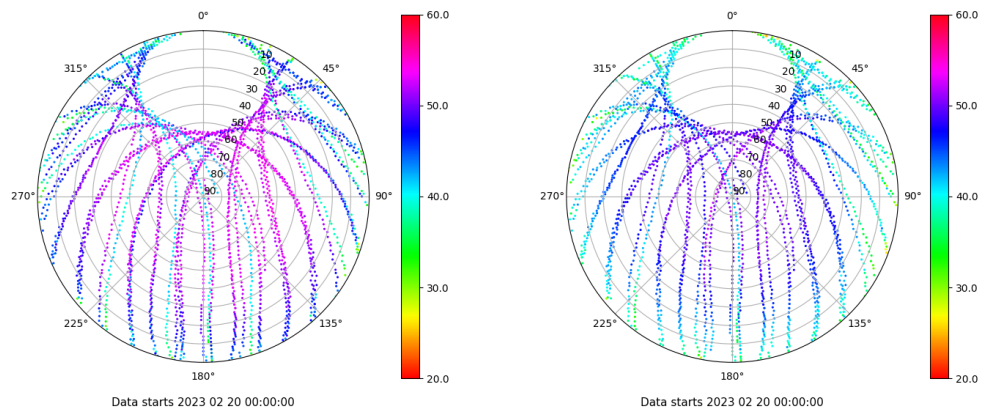
Skyplot for station ALBA. Signal to Noise S1C Data file ALBA00ESP_R_2023051.xtr Skyplot for station ALBA. Signal to Noise S2C Data file ALBA00ESP_R_2023051.xtr
