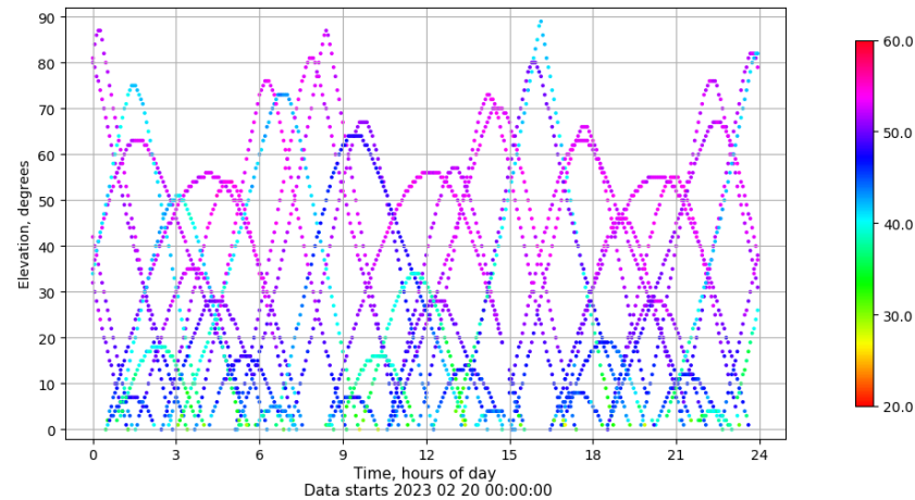
Time-elevation plot for station ALBA. Signal to Noise S1C Data file ALBA00ESP_R_2023051.xtr
