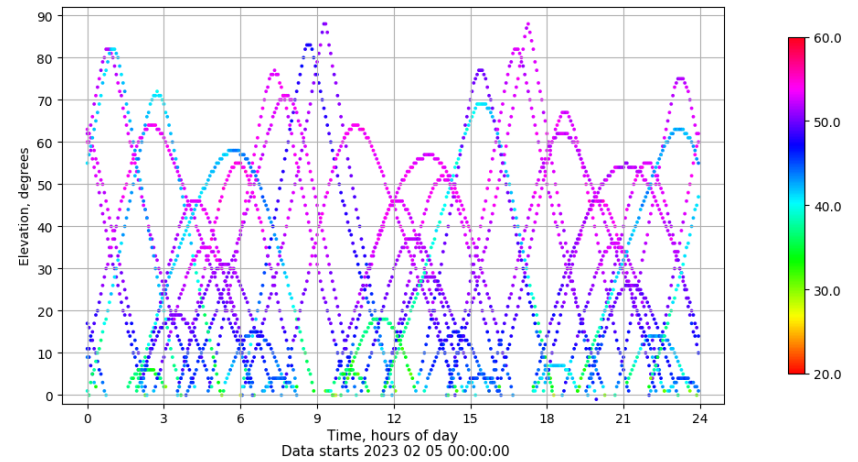
Time-elevation plot for station ALBA. Signal to Noise S1C Data file ALBA00ESP_R_2023036.xtr
