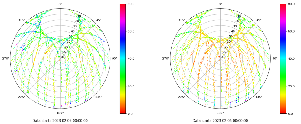
Skyplot for station ALBA. Parameter M1C Data file ALBA00ESP_R_2023036.xtr Skyplot for station ALBA. Parameter M2C Data file ALBA00ESP_R_2023036.xtr
