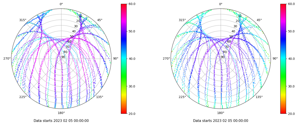
Skyplot for station ALBA. Signal to Noise S1C Data file ALBA00ESP_R_2023036.xtr Skyplot for station ALBA. Signal to Noise S2C Data file ALBA00ESP_R_2023036.xtr
