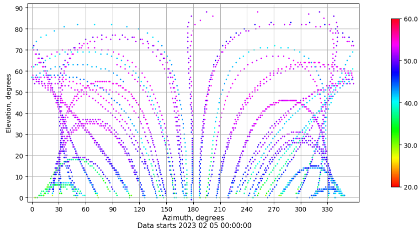
Azimuth-elevation plot for station ALBA. Signal to Noise S1C Data file ALBA00ESP_R_2023036.xtr
