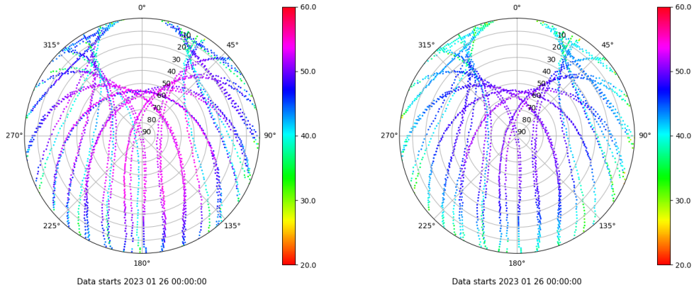
Skyplot for station ALBA. Signal to Noise S1C Data file ALBA00ESP_R_2023026.xtr Skyplot for station ALBA. Signal to Noise S2C Data file ALBA00ESP_R_2023026.xtr
