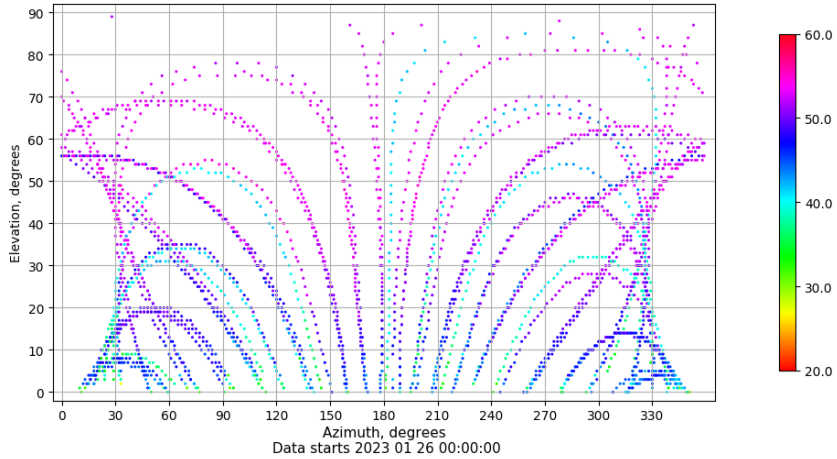
Azimuth-elevation plot for station ALBA. Signal to Noise S1C Data file ALBA00ESP_R_2023026.xtr
