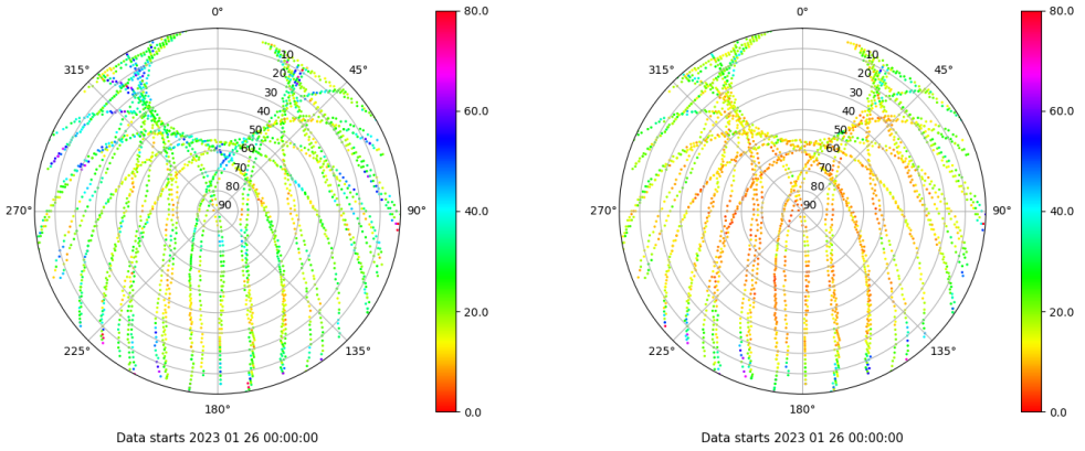
Skyplot for station ALBA. Parameter M1C Data file ALBA00ESP_R_2023026.xtr Skyplot for station ALBA. Parameter M2C Data file ALBA00ESP_R_2023026.xtr
