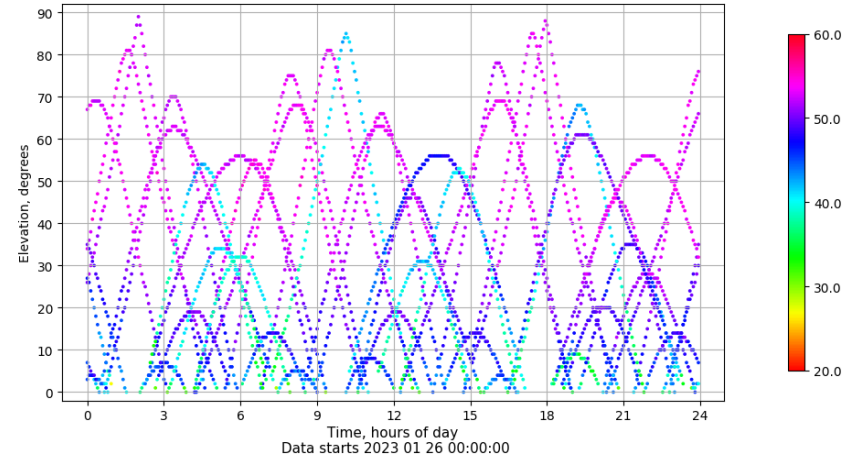
Time-elevation plot for station ALBA. Signal to Noise S1C Data file ALBA00ESP_R_2023026.xtr
