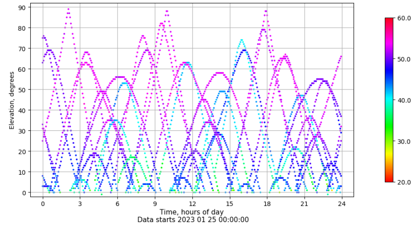
Time-elevation plot for station ALBA. Signal to Noise S1C Data file ALBA00ESP_R_2023025.xtr
