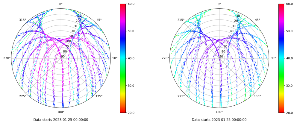
Skyplot for station ALBA. Signal to Noise S1C Data file ALBA00ESP_R_2023025.xtr Skyplot for station ALBA. Signal to Noise S2C Data file ALBA00ESP_R_2023025.xtr
