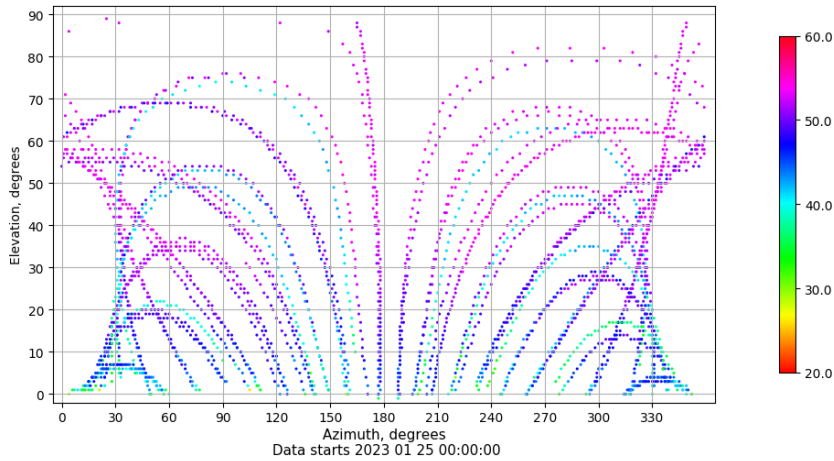
Azimuth-elevation plot for station ALBA. Signal to Noise S1C Data file ALBA00ESP_R_2023025.xtr
