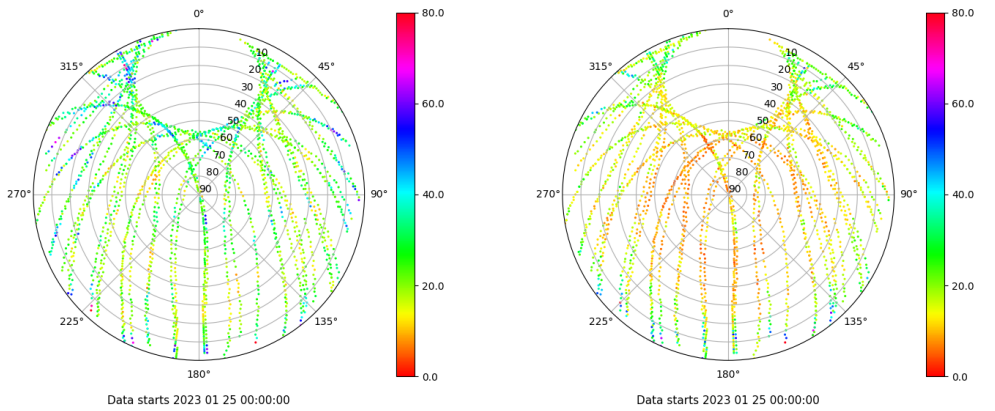
Skyplot for station ALBA. Parameter M1C Data file ALBA00ESP_R_2023025.xtr Skyplot for station ALBA. Parameter M2C Data file ALBA00ESP_R_2023025.xtr
