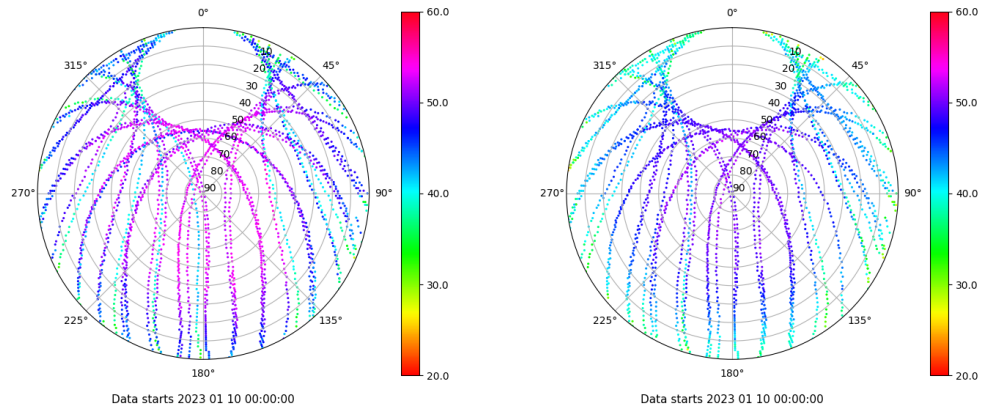
Skyplot for station ALBA. Signal to Noise S1C Data file ALBA00ESP_R_2023010.xtr Skyplot for station ALBA. Signal to Noise S2C Data file ALBA00ESP_R_2023010.xtr
