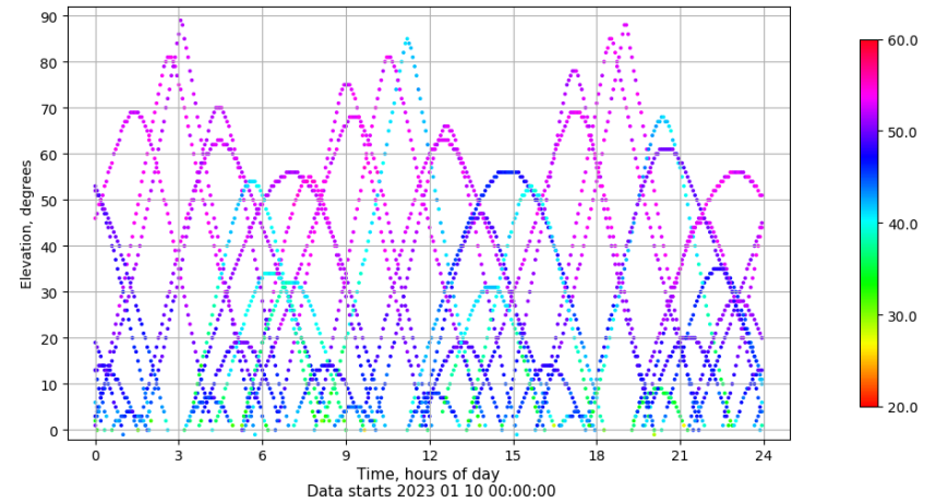
Time-elevation plot for station ALBA. Signal to Noise S1C Data file ALBA00ESP_R_2023010.xtr
