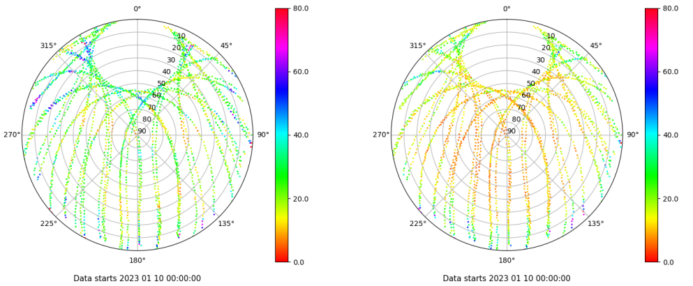
Skyplot for station ALBA. Parameter M1C Data file ALBA00ESP_R_2023010.xtr Skyplot for station ALBA. Parameter M2C Data file ALBA00ESP_R_2023010.xtr
