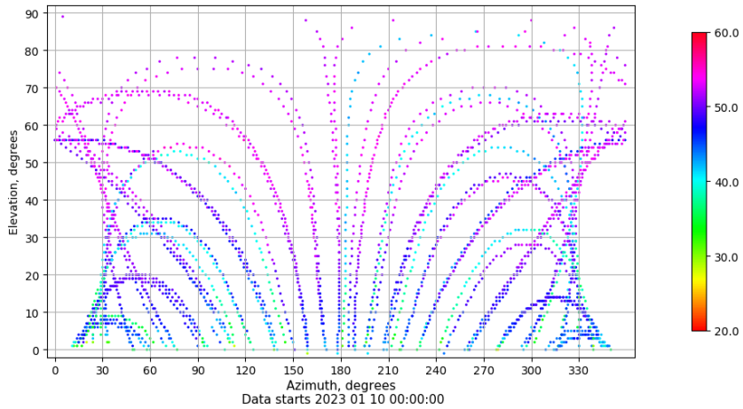
Azimuth-elevation plot for station ALBA. Signal to Noise S1C Data file ALBA00ESP_R_2023010.xtr
