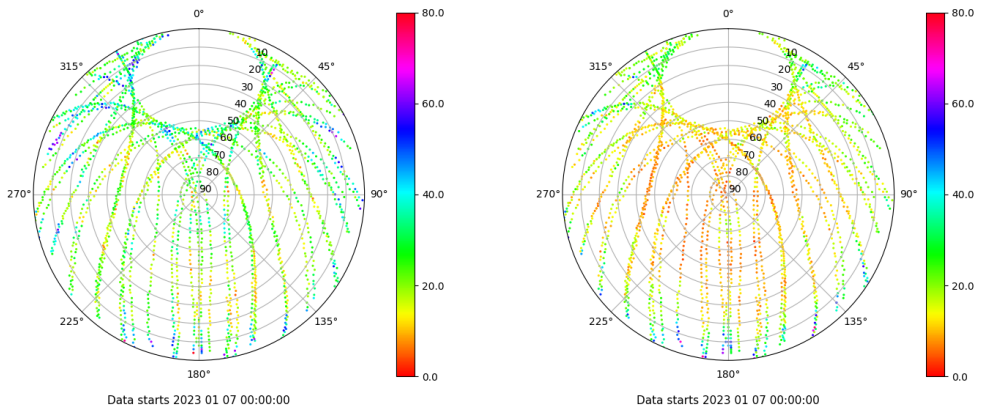
Skyplot for station ALBA. Parameter M1C Data file ALBA00ESP_R_2023007.xtr Skyplot for station ALBA. Parameter M2C Data file ALBA00ESP_R_2023007.xtr
