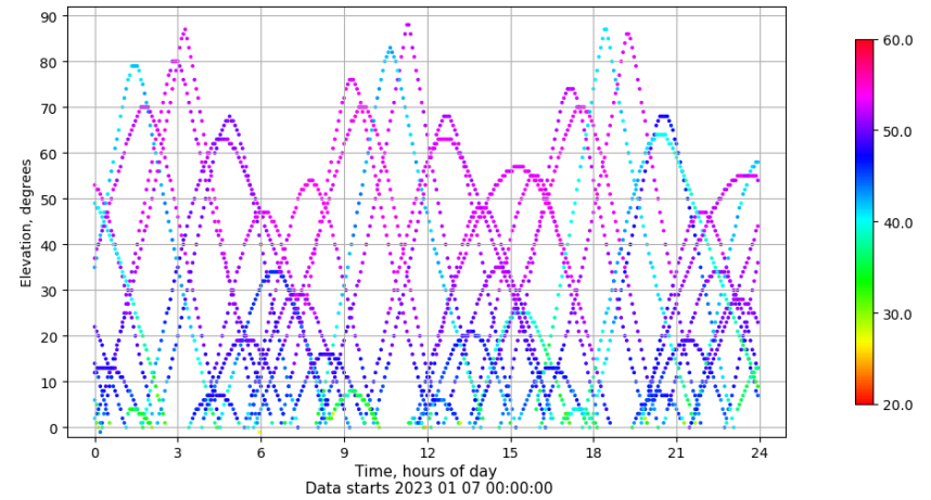
Time-elevation plot for station ALBA. Signal to Noise S1C Data file ALBA00ESP_R_2023007.xtr
