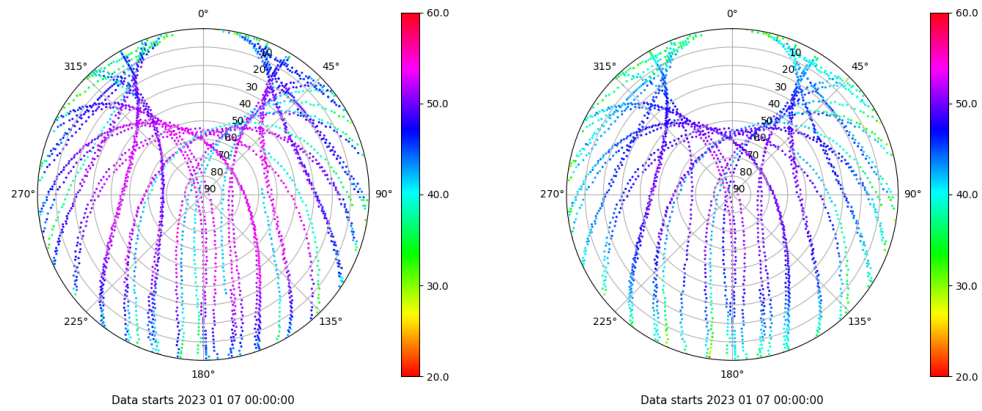
Skyplot for station ALBA. Signal to Noise S1C Data file ALBA00ESP_R_2023007.xtr Skyplot for station ALBA. Signal to Noise S2C Data file ALBA00ESP_R_2023007.xtr
