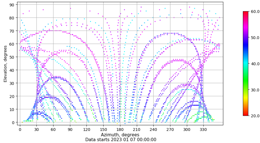
Azimuth-elevation plot for station ALBA. Signal to Noise S1C Data file ALBA00ESP_R_2023007.xtr
