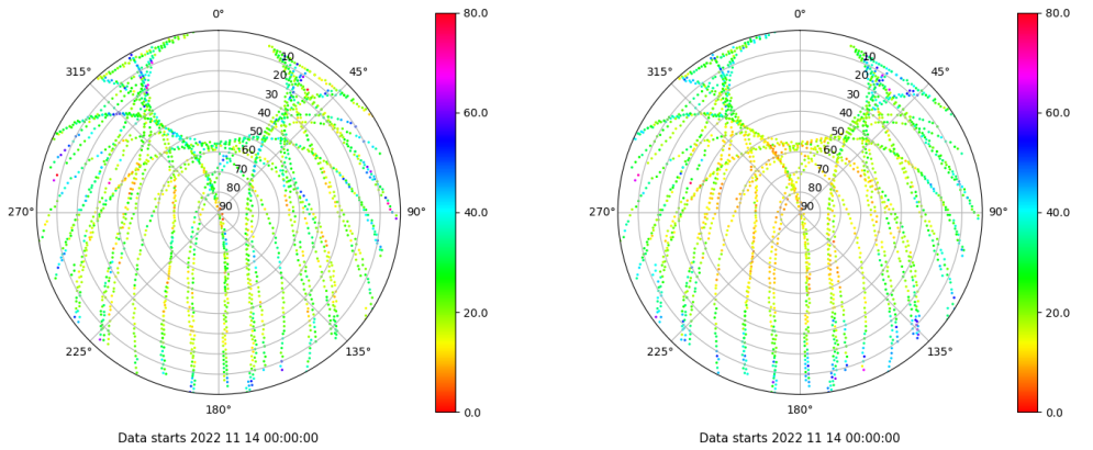
Skyplot for station ALBA. Parameter M1C Data file ALBA00ESP_R_2022318.xtr Skyplot for station ALBA. Parameter M2P Data file ALBA00ESP_R_2022318.xtr
