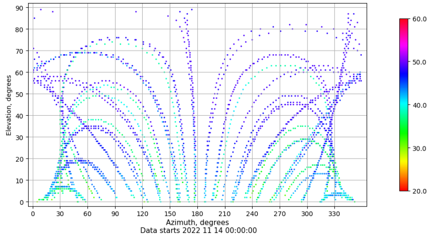
Azimuth-elevation plot for station ALBA. Signal to Noise S1C Data file ALBA00ESP_R_2022318.xtr
