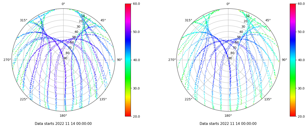
Skyplot for station ALBA. Signal to Noise S1C Data file ALBA00ESP_R_2022318.xtr Skyplot for station ALBA. Signal to Noise S2P Data file ALBA00ESP_R_2022318.xtr
