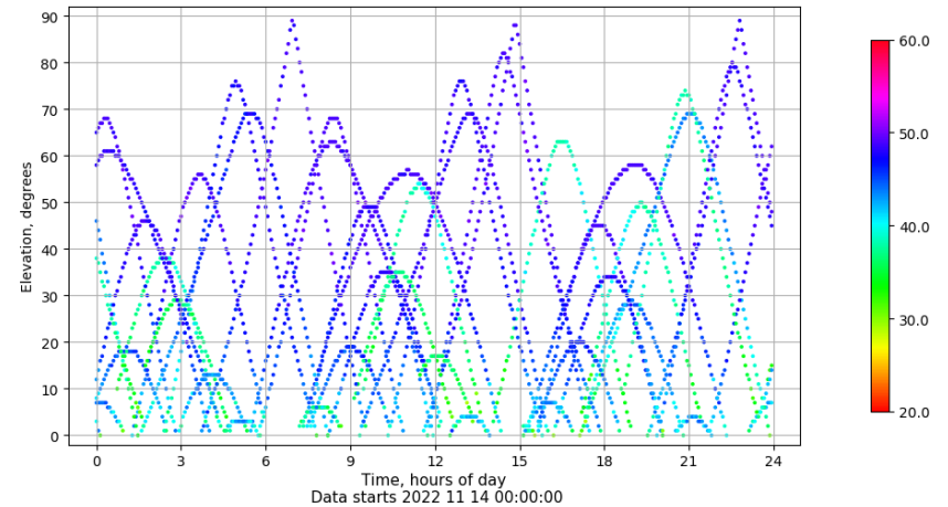
Time-elevation plot for station ALBA. Signal to Noise S1C Data file ALBA00ESP_R_2022318.xtr
