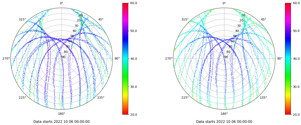
Skyplot for station ALBA. Signal to Noise S1C Data file ALBA00ESP_R_2022279.xtr Skyplot for station ALBA. Signal to Noise S2P Data file ALBA00ESP_R_2022279.xtr
