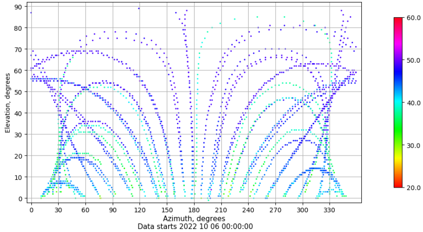
Azimuth-elevation plot for station ALBA. Signal to Noise S1C Data file ALBA00ESP_R_2022279.xtr
