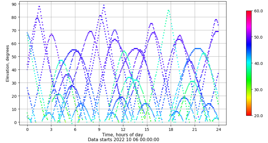
Time-elevation plot for station ALBA. Signal to Noise S1C Data file ALBA00ESP_R_2022279.xtr
