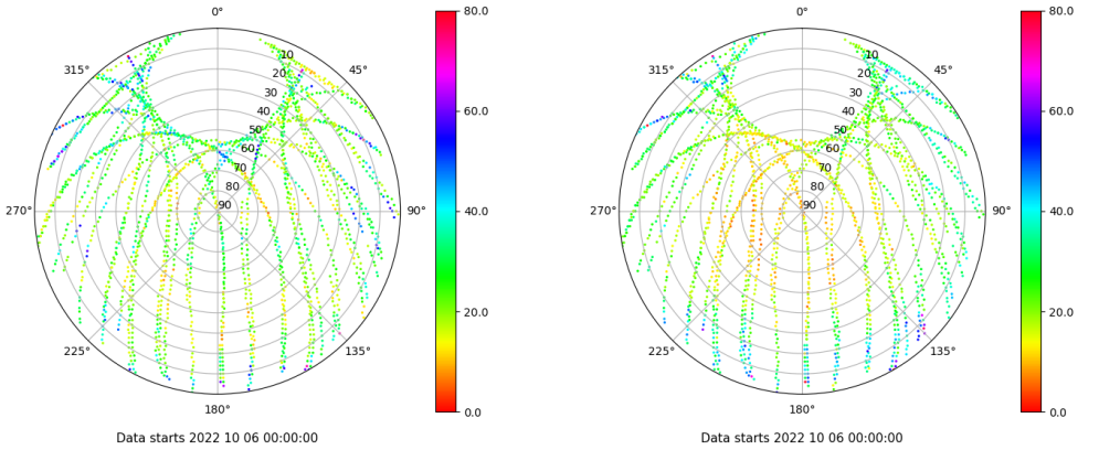
Skyplot for station ALBA. Parameter M1C Data file ALBA00ESP_R_2022279.xtr Skyplot for station ALBA. Parameter M2P Data file ALBA00ESP_R_2022279.xtr
