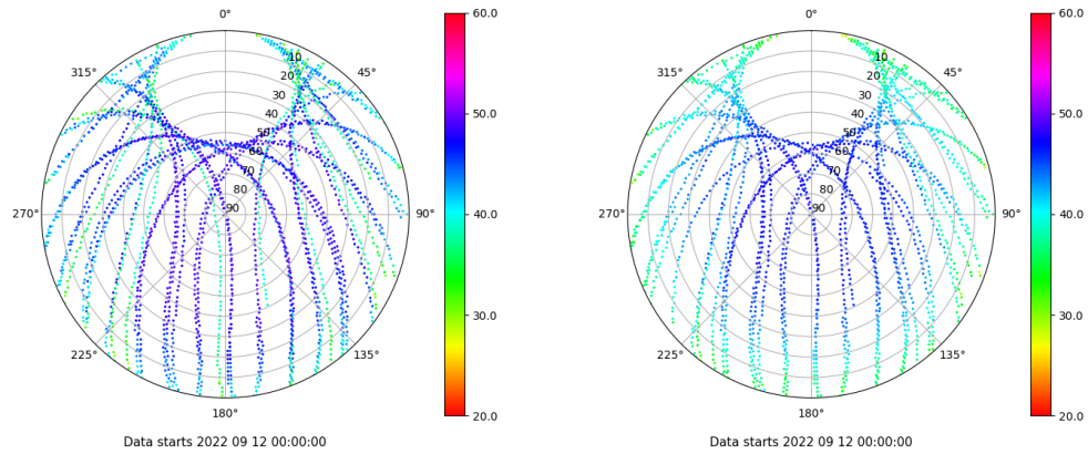
Skyplot for station ALBA. Signal to Noise S1C Data file ALBA00ESP_R_2022255.xtr Skyplot for station ALBA. Signal to Noise S2P Data file ALBA00ESP_R_2022255.xtr
