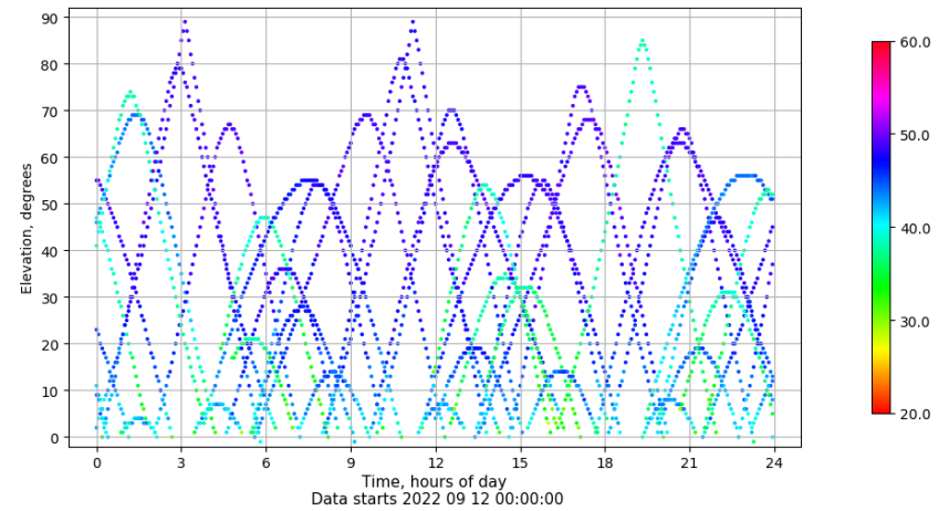
Time-elevation plot for station ALBA. Signal to Noise S1C Data file ALBA00ESP_R_2022255.xtr
