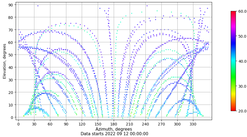
Azimuth-elevation plot for station ALBA. Signal to Noise S1C Data file ALBA00ESP_R_2022255.xtr
