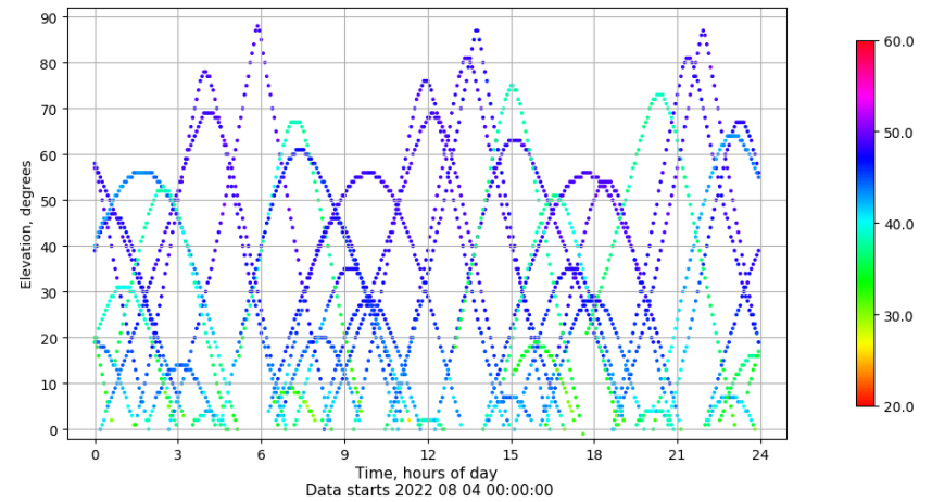
Time-elevation plot for station ALBA. Signal to Noise S1C Data file ALBA00ESP_R_2022216.xtr
