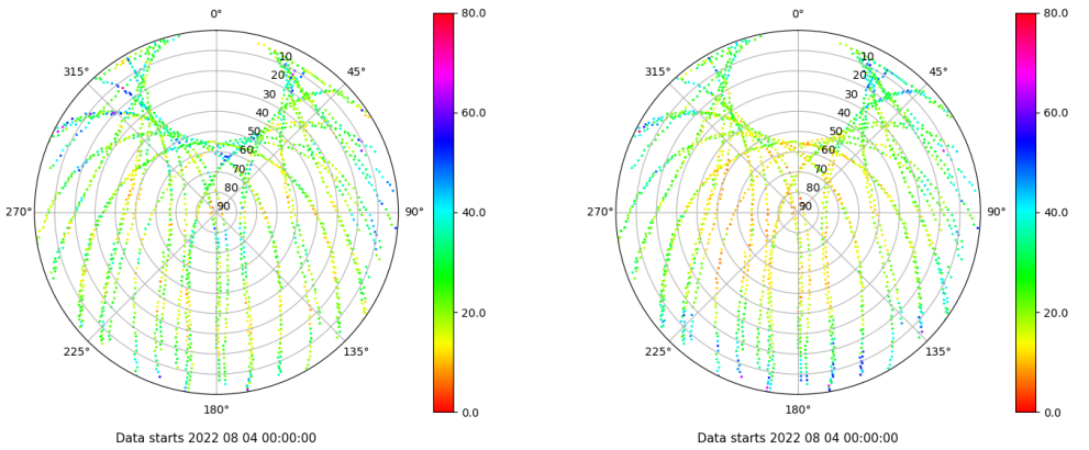
Skyplot for station ALBA. Parameter M1C Data file ALBA00ESP_R_2022216.xtr Skyplot for station ALBA. Parameter M2P Data file ALBA00ESP_R_2022216.xtr
