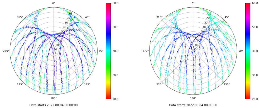
Skyplot for station ALBA. Signal to Noise S1C Data file ALBA00ESP_R_2022216.xtr Skyplot for station ALBA. Signal to Noise S2P Data file ALBA00ESP_R_2022216.xtr
