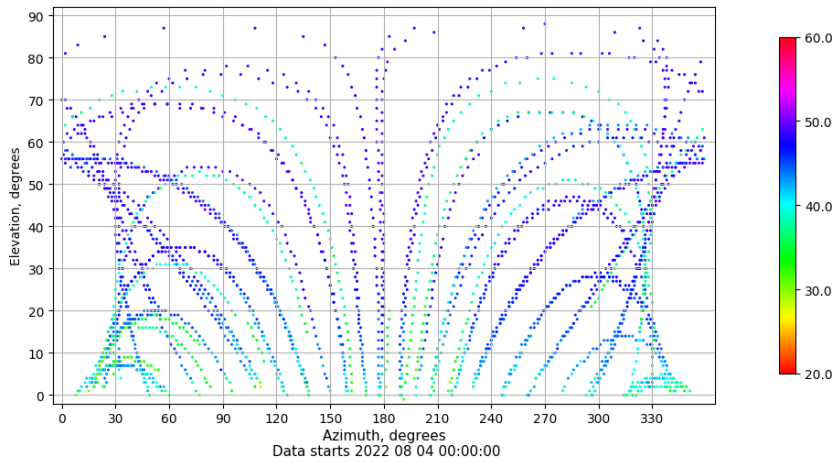
Azimuth-elevation plot for station ALBA. Signal to Noise S1C Data file ALBA00ESP_R_2022216.xtr
