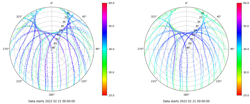
Skyplot for station ALBA. Signal to Noise S1C Data file ALBA00ESP_R_2022052.xtr Skyplot for station ALBA. Signal to Noise S2P Data file ALBA00ESP_R_2022052.xtr
