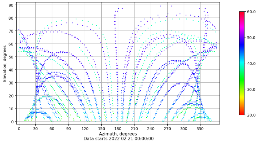
Azimuth-elevation plot for station ALBA. Signal to Noise S1C Data file ALBA00ESP_R_2022052.xtr
