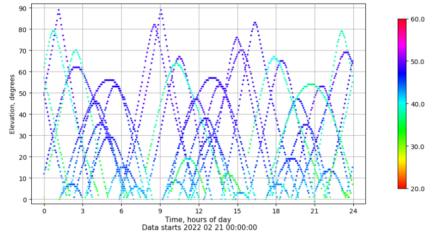
Time-elevation plot for station ALBA. Signal to Noise S1C Data file ALBA00ESP_R_2022052.xtr
