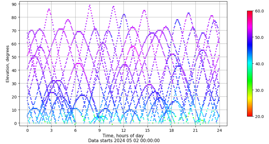
Time-elevation plot for station ALAC. Signal to Noise S1C Data file ALAC00ESP_R_2024123.xtr
