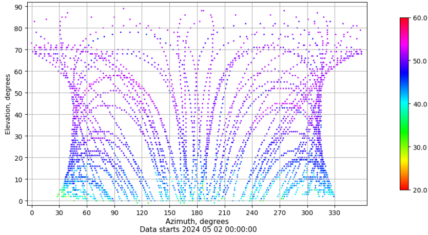
Azimuth-elevation plot for station ALAC. Signal to Noise S1C Data file ALAC00ESP_R_2024123.xtr
