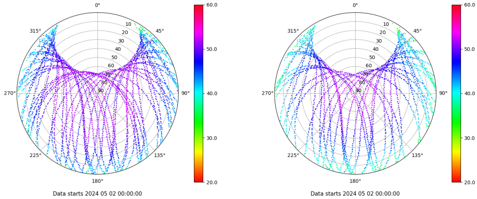
Skyplot for station ALAC. Signal to Noise S1C Data file ALAC00ESP_R_2024123.xtr Skyplot for station ALAC. Signal to Noise S2S Data file ALAC00ESP_R_2024123.xtr
