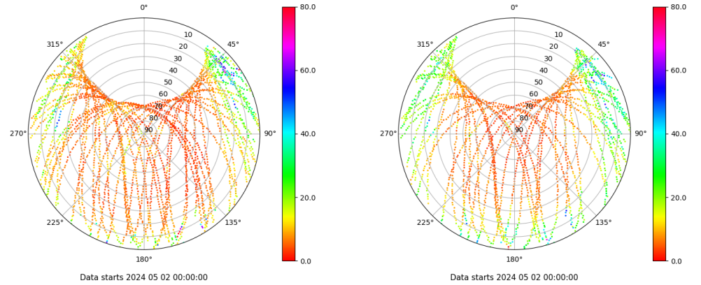
Skyplot for station ALAC. Parameter M1C Data file ALAC00ESP_R_2024123.xtr Skyplot for station ALAC. Parameter M2S Data file ALAC00ESP_R_2024123.xtr
