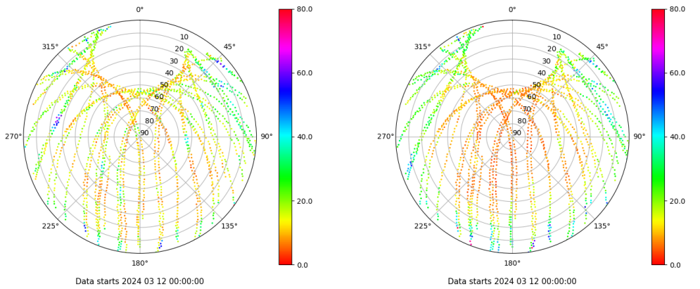
Skyplot for station ALAC. Parameter M1C Data file ALAC00ESP_R_2024072.xtr Skyplot for station ALAC. Parameter M2P Data file ALAC00ESP_R_2024072.xtr
