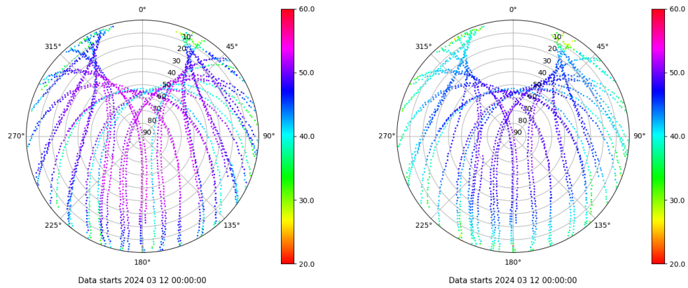
Skyplot for station ALAC. Signal to Noise S1C Data file ALAC00ESP_R_2024072.xtr Skyplot for station ALAC. Signal to Noise S2P Data file ALAC00ESP_R_2024072.xtr
