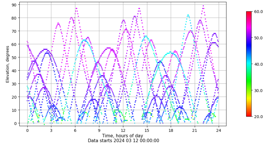
Time-elevation plot for station ALAC. Signal to Noise S1C Data file ALAC00ESP_R_2024072.xtr
