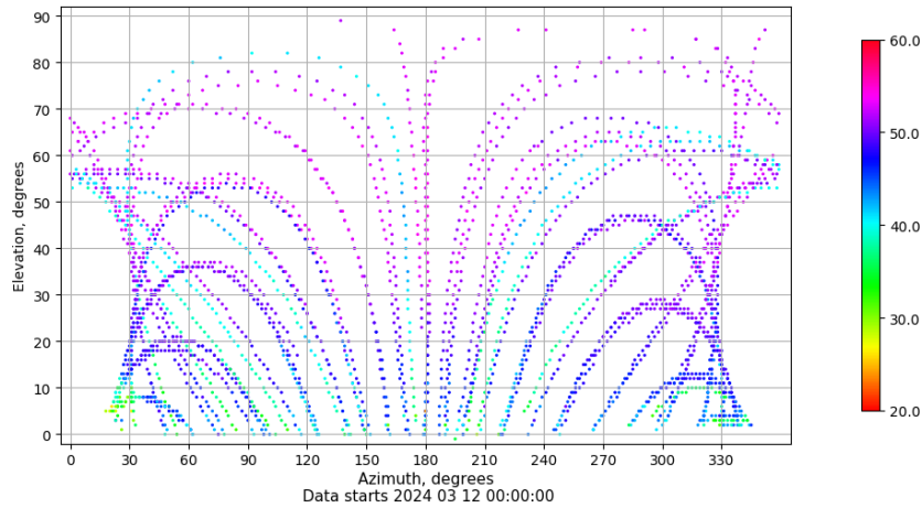
Azimuth-elevation plot for station ALAC. Signal to Noise S1C Data file ALAC00ESP_R_2024072.xtr
