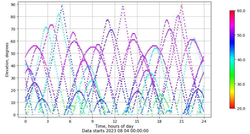
Time-elevation plot for station ALAC. Signal to Noise S1C Data file ALAC00ESP_R_2023216.xtr
