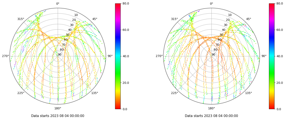
Skyplot for station ALAC. Parameter M1C Data file ALAC00ESP_R_2023216.xtr Skyplot for station ALAC. Parameter M2P Data file ALAC00ESP_R_2023216.xtr
