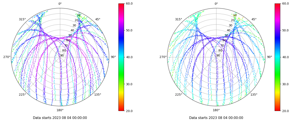
Skyplot for station ALAC. Signal to Noise S1C Data file ALAC00ESP_R_2023216.xtr Skyplot for station ALAC. Signal to Noise S2P Data file ALAC00ESP_R_2023216.xtr
