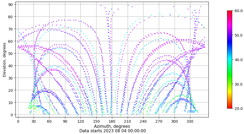
Azimuth-elevation plot for station ALAC. Signal to Noise S1C Data file ALAC00ESP_R_2023216.xtr
