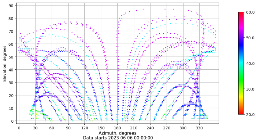
Azimuth-elevation plot for station ALAC. Signal to Noise S1C Data file ALAC00ESP_R_2023157.xtr
