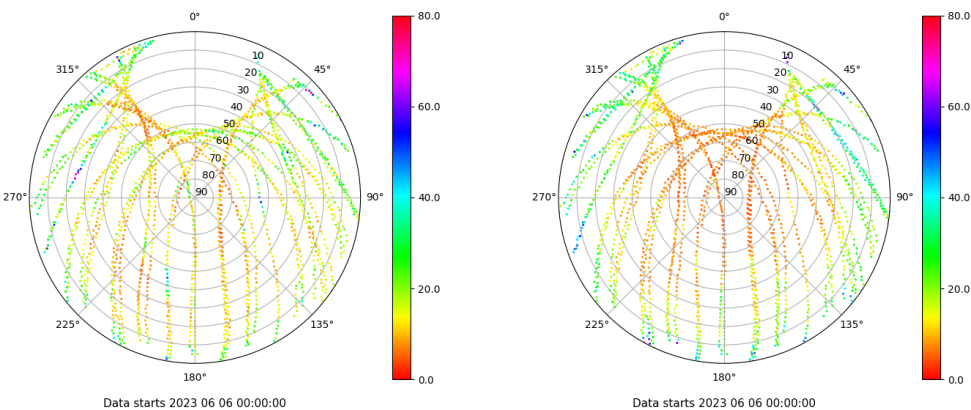
Skyplot for station ALAC. Parameter M1C Data file ALAC00ESP_R_2023157.xtr Skyplot for station ALAC. Parameter M2P Data file ALAC00ESP_R_2023157.xtr
