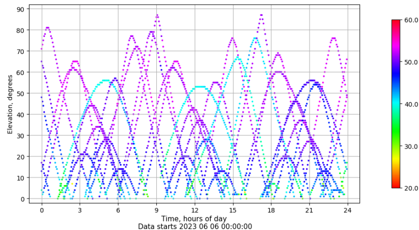
Time-elevation plot for station ALAC. Signal to Noise S1C Data file ALAC00ESP_R_2023157.xtr
