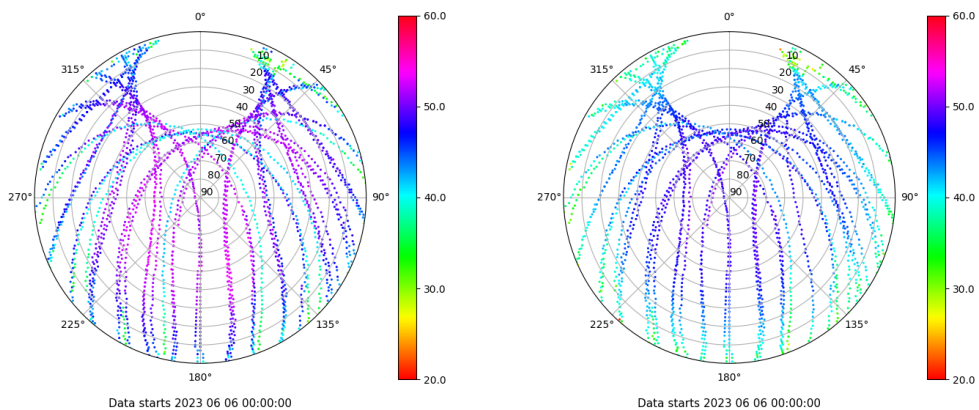
Skyplot for station ALAC. Signal to Noise S1C Data file ALAC00ESP_R_2023157.xtr Skyplot for station ALAC. Signal to Noise S2P Data file ALAC00ESP_R_2023157.xtr
