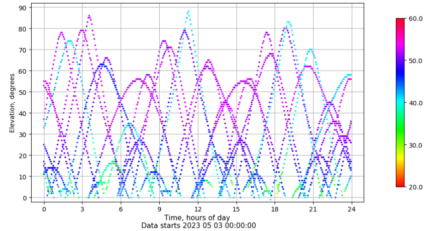
Time-elevation plot for station ALAC. Signal to Noise S1C Data file ALAC00ESP_R_2023123.xtr
