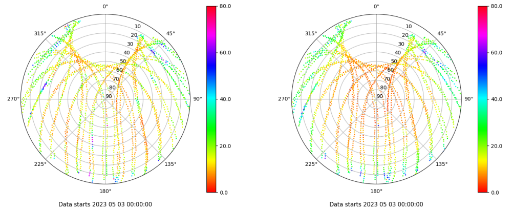
Skyplot for station ALAC. Parameter M1C Data file ALAC00ESP_R_2023123.xtr Skyplot for station ALAC. Parameter M2P Data file ALAC00ESP_R_2023123.xtr
