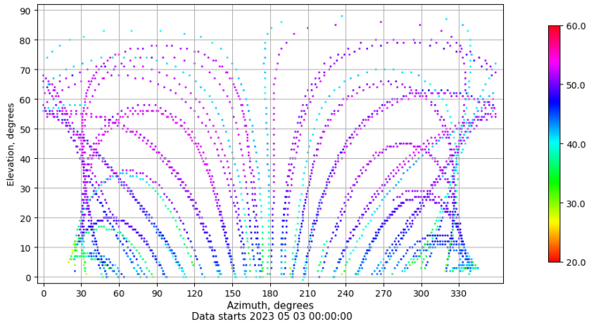
Azimuth-elevation plot for station ALAC. Signal to Noise S1C Data file ALAC00ESP_R_2023123.xtr
