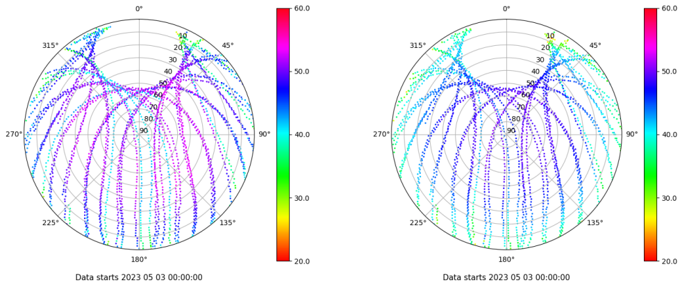
Skyplot for station ALAC. Signal to Noise S1C Data file ALAC00ESP_R_2023123.xtr Skyplot for station ALAC. Signal to Noise S2P Data file ALAC00ESP_R_2023123.xtr
