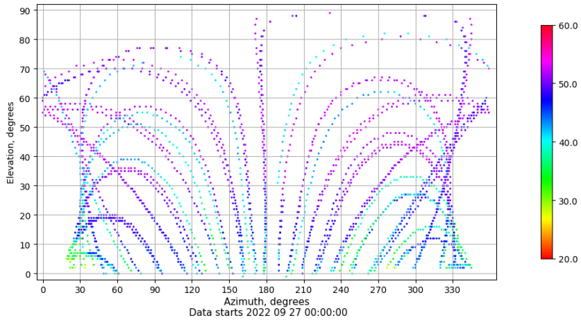
Azimuth-elevation plot for station ALAC. Signal to Noise S1C Data file ALAC00ESP_R_2022270.xtr
