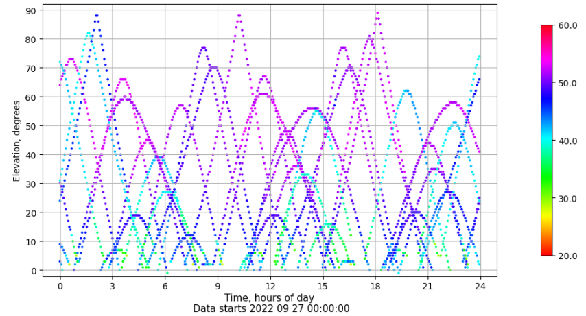
Time-elevation plot for station ALAC. Signal to Noise S1C Data file ALAC00ESP_R_2022270.xtr
