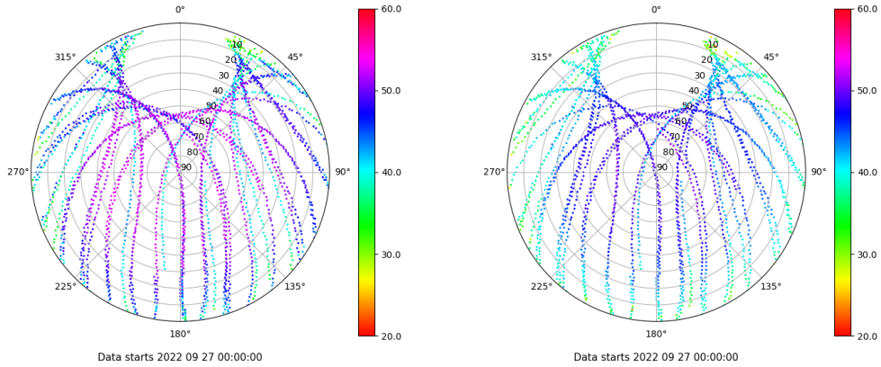
Skyplot for station ALAC. Signal to Noise S1C Data file ALAC00ESP_R_2022270.xtr Skyplot for station ALAC. Signal to Noise S2P Data file ALAC00ESP_R_2022270.xtr
