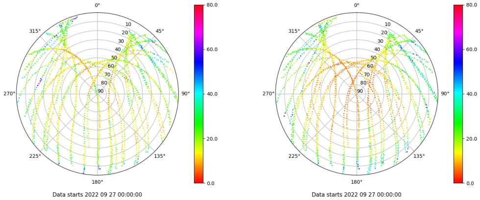
Skyplot for station ALAC. Parameter M1C Data file ALAC00ESP_R_2022270.xtr Skyplot for station ALAC. Parameter M2P Data file ALAC00ESP_R_2022270.xtr
