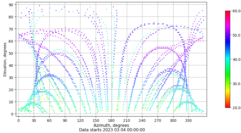
Azimuth-elevation plot for station ACOR. Signal to Noise S1C Data file ACOR00ESP_R_2023063.xtr
