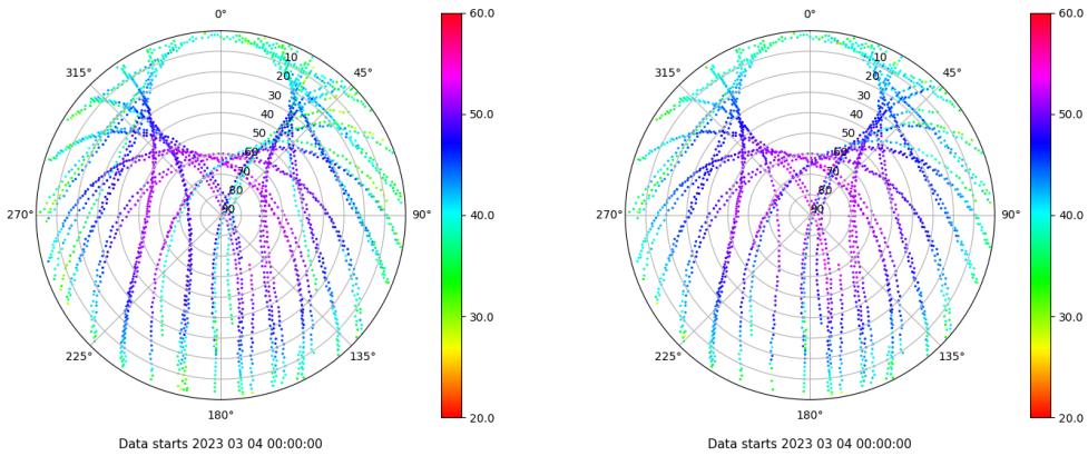
Skyplot for station ACOR. Signal to Noise S1C Data file ACOR00ESP_R_2023063.xtr Skyplot for station ACOR. Signal to Noise S2C Data file ACOR00ESP_R_2023063.xtr
