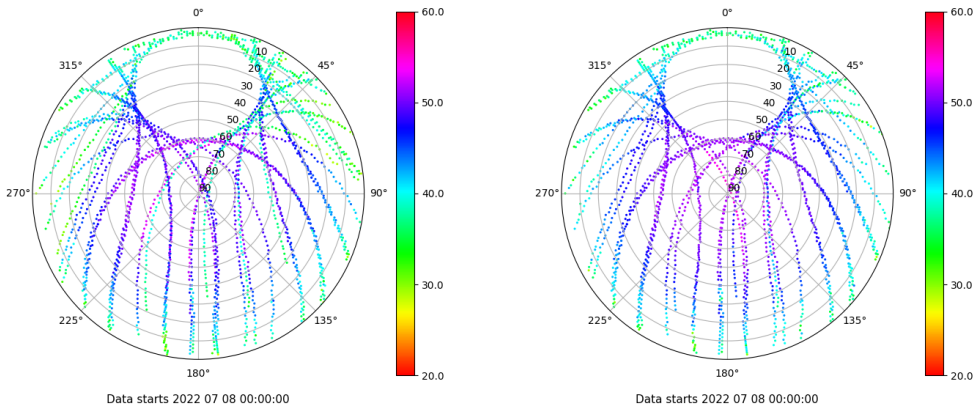
Skyplot for station ACOR. Signal to Noise S1C Data file ACOR00ESP_R_2022189.xtr Skyplot for station ACOR. Signal to Noise S2C Data file ACOR00ESP_R_2022189.xtr
