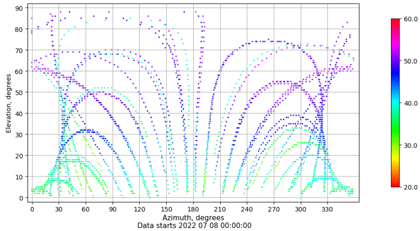
Azimuth-elevation plot for station ACOR. Signal to Noise S1C Data file ACOR00ESP_R_2022189.xtr
