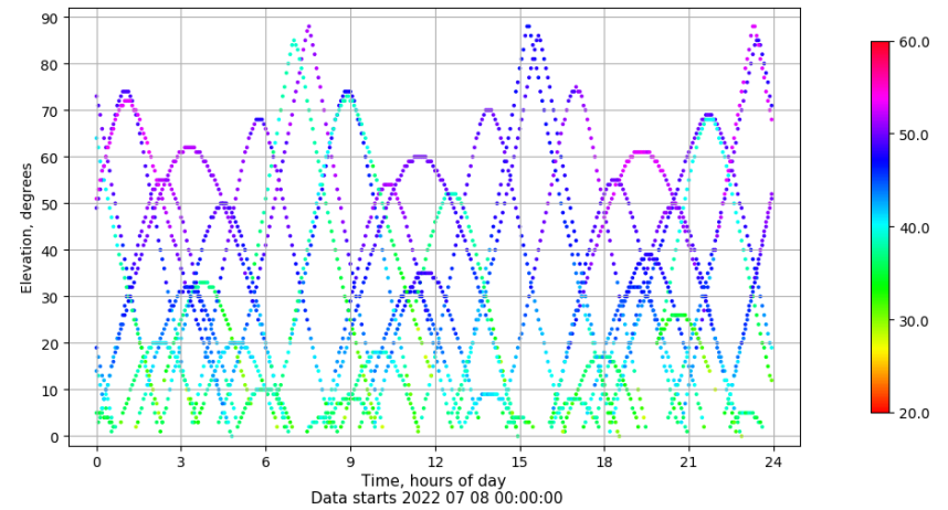
Time-elevation plot for station ACOR. Signal to Noise S1C Data file ACOR00ESP_R_2022189.xtr
